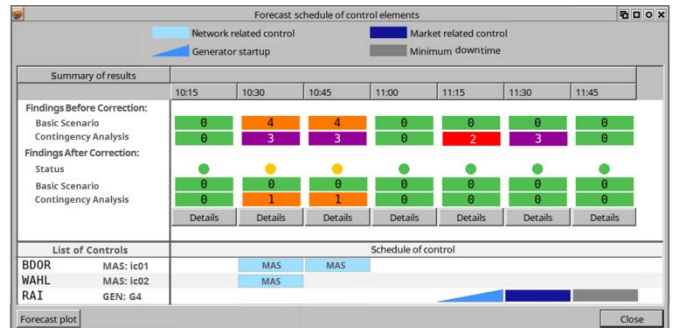
Figure 4: Exemplary Snapshot of Control Actions under Consideration of DPFCs and MAS in PSIconrol
