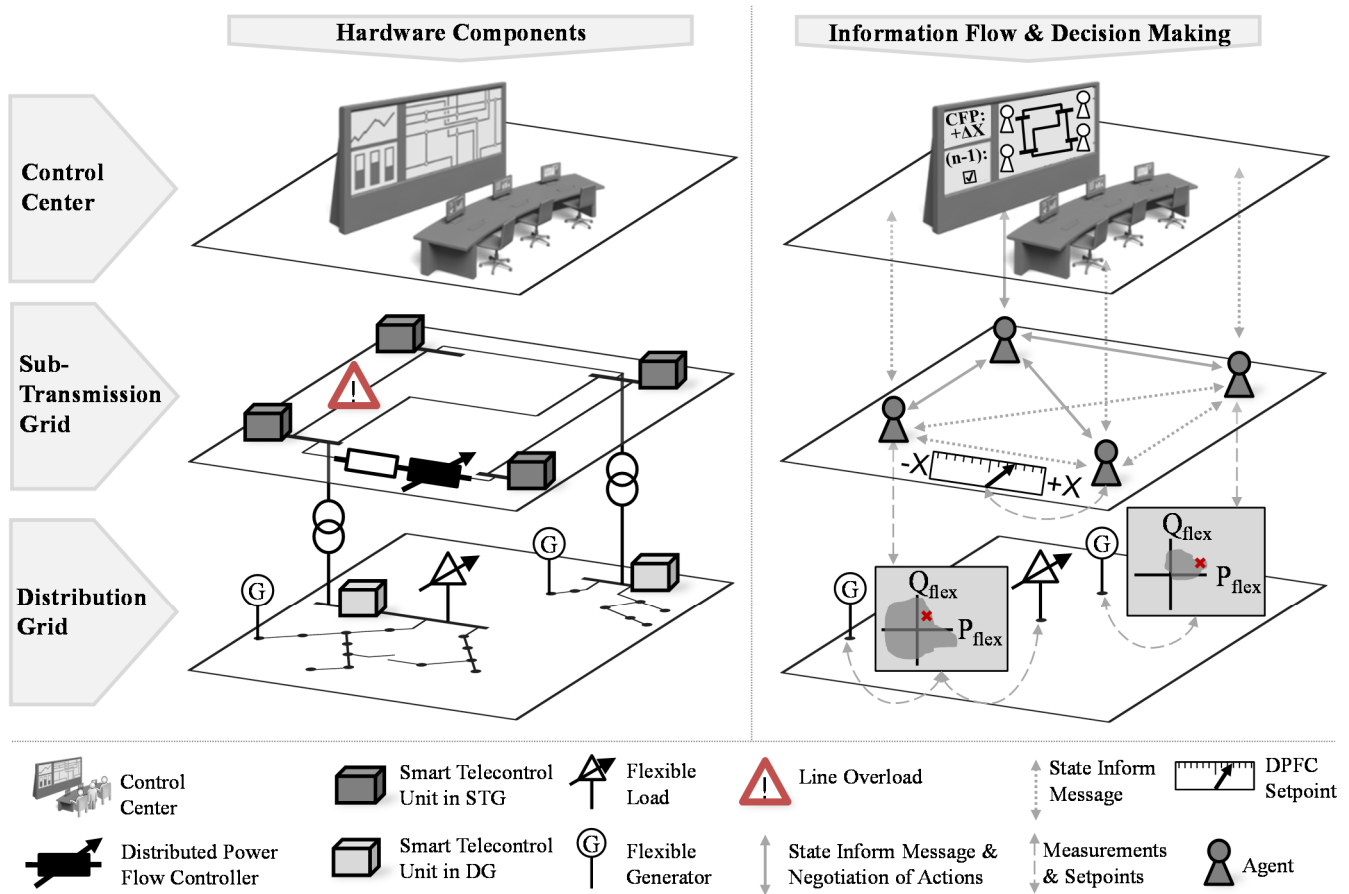
Figure 2: Overview of the System Concept of the IDEAL-Project
