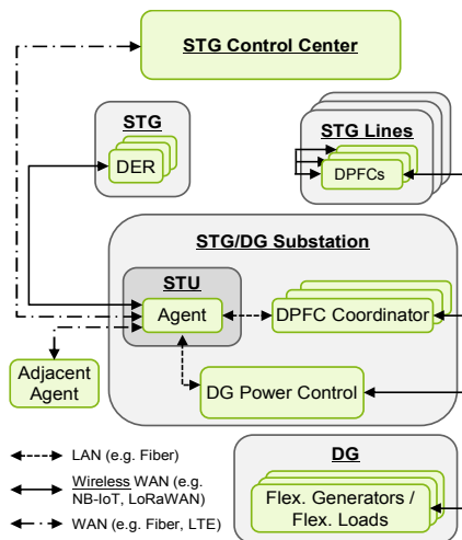
Figure 1: Overview of communication links between system components
