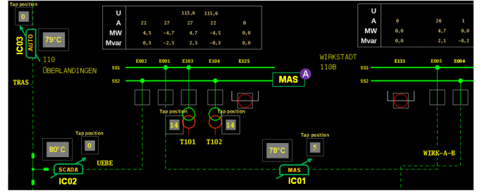
Figure 3: Process visualization of MAS and DPFCs embedded in an exemplary 110 kV grid in PSIconrol
